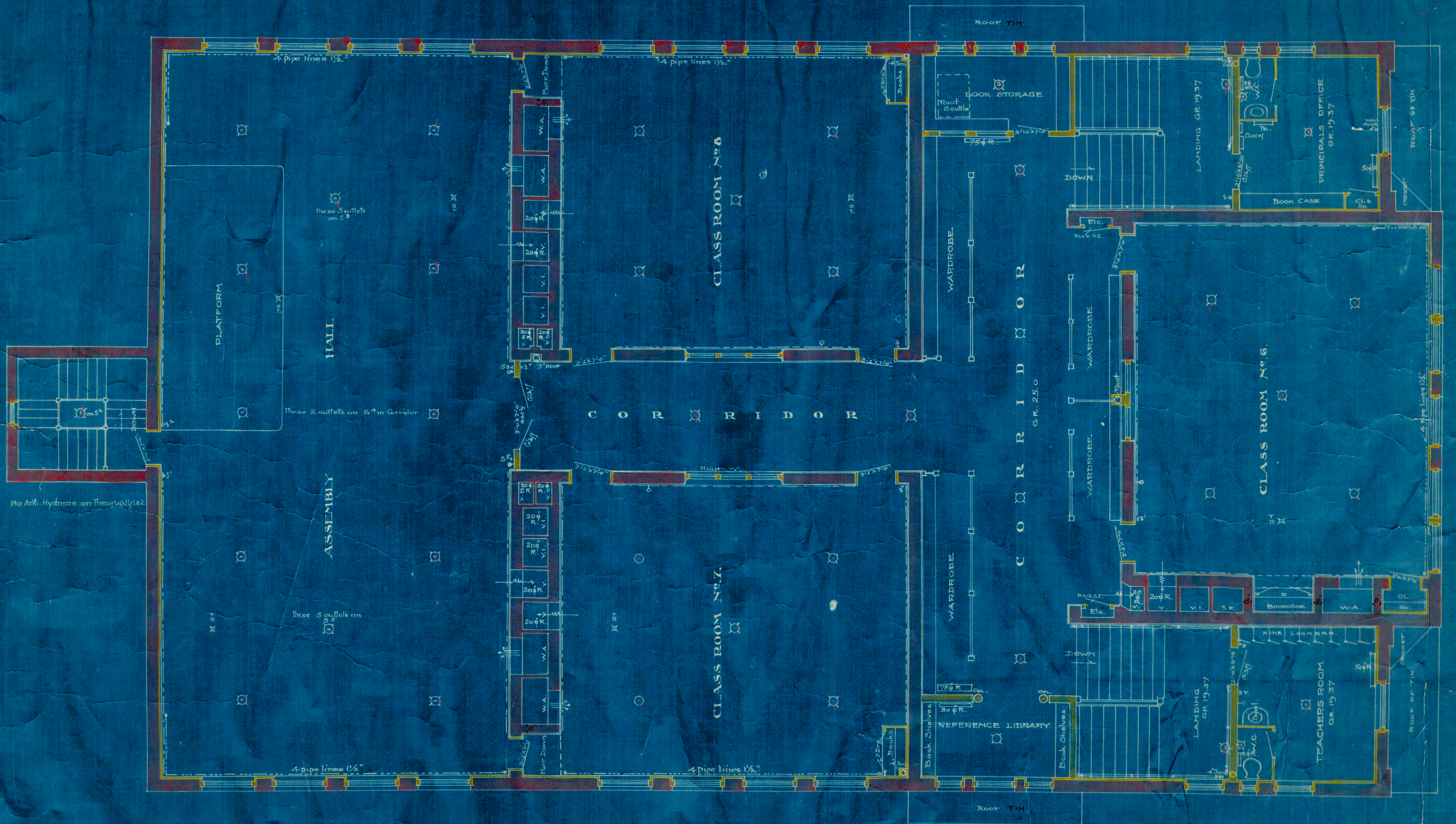
SECOND FLOOR PLAN SCALE 1/4" = ONE FOOT
